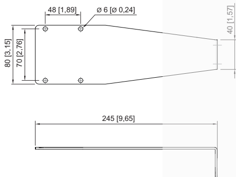
Mounting plate
