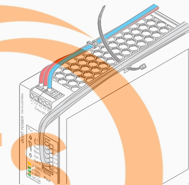
Figure 14 Lay and align connection wiring
