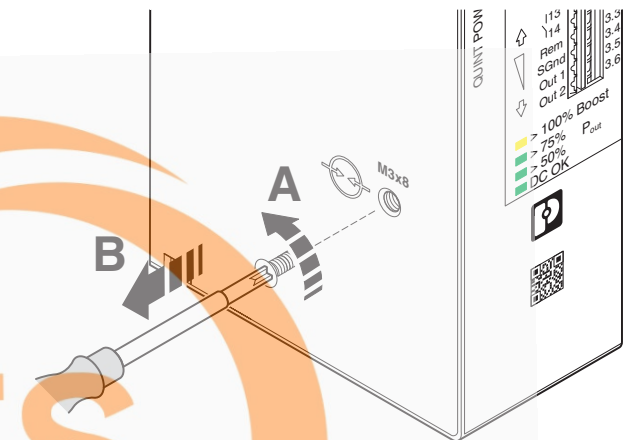
Figure 2 Disconnect gas discharge tube
