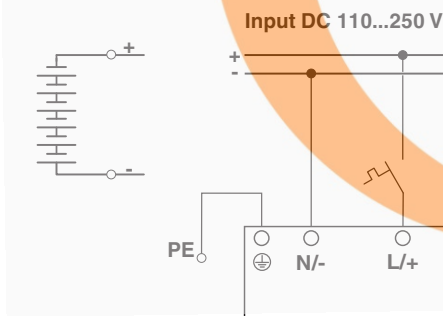
Figure 19 Pin assignment for DC supply voltage
