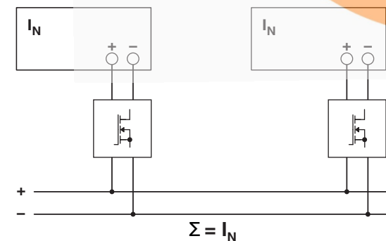
Figure 47 Schematic diagram, redundant operation with QUINT S-ORING
