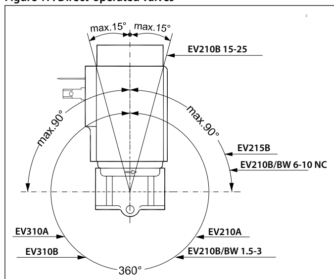
Figure 17: Direct-operated valves
