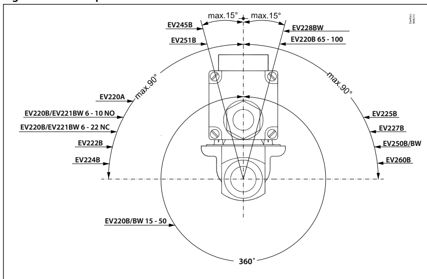
Figure 15: servo-operated valves
