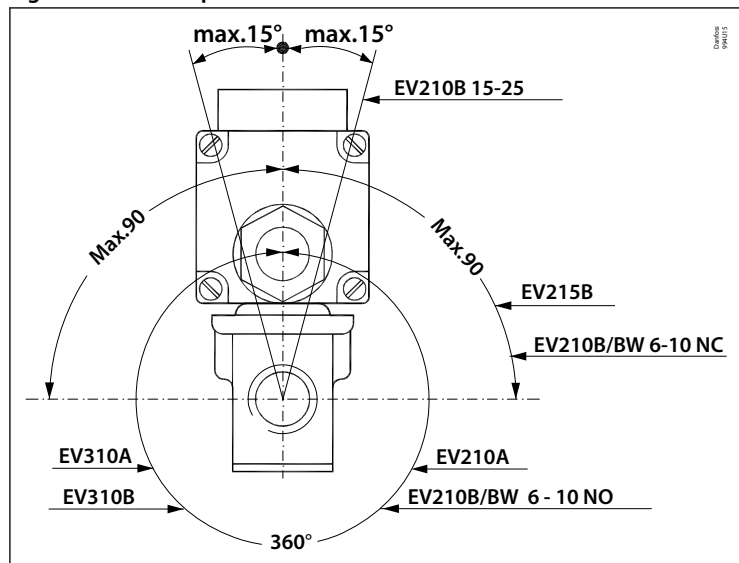
Figure 17: Direct-operated valves
