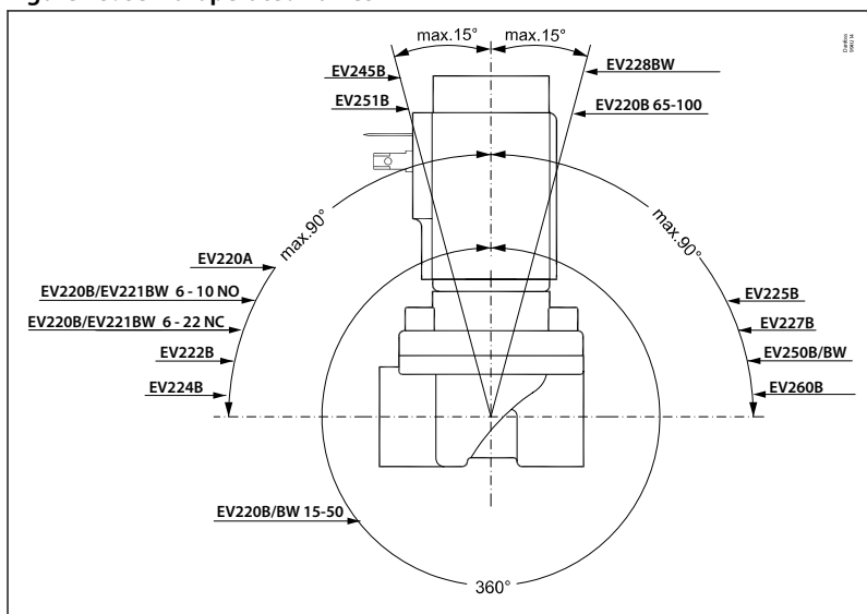
Figure 15: servo-operated valves
