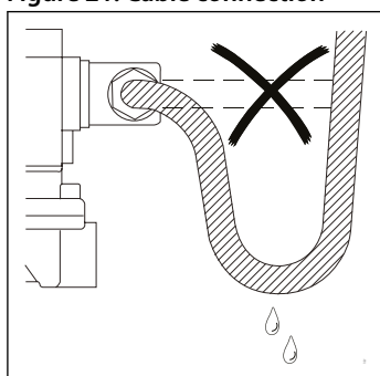
Figure 21: Cable connection
