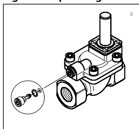
Figure 9: Equalizing orifice
