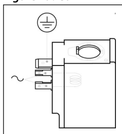
Figure 19: Coil
