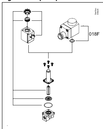
Figure 33: Spare parts set
