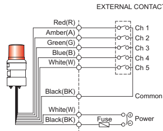
STND100R/STND100L/STND100LR-DC/AC
