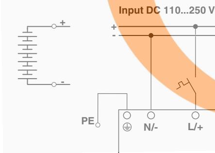
Figure 19 Pin assignment for DC supply voltage
