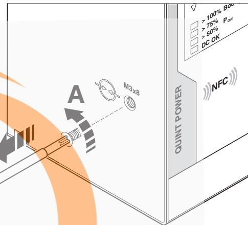
Figure 2 Disconnect gas-filled surge arrester
