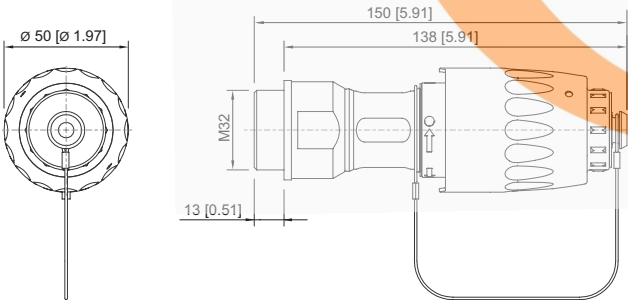
8595/1 bulkhead plug
