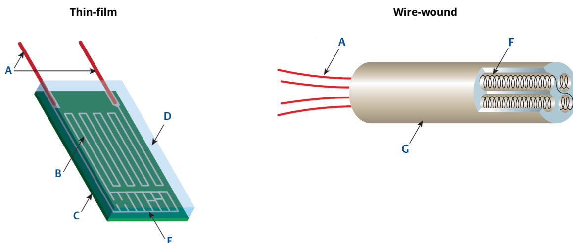
Figure 3: RTD Elements
