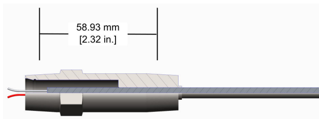
Figure 16: Dimensions
