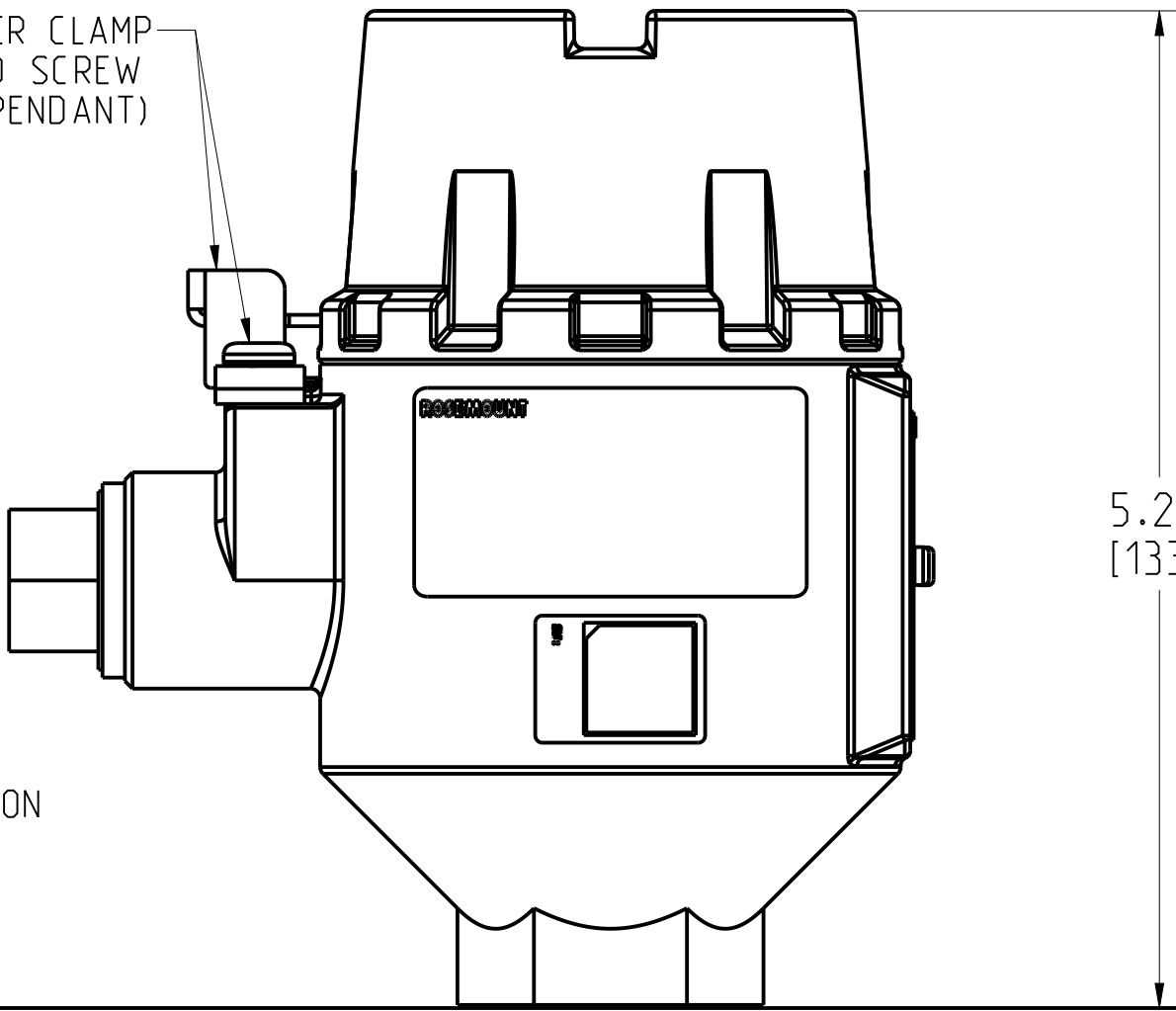
ROSEMOUNT ALUMINUM WITH DISPLAY COVER (AR2) OR SST ROSEMOUNT SST WITH DISPLAY COVER (SR2)
