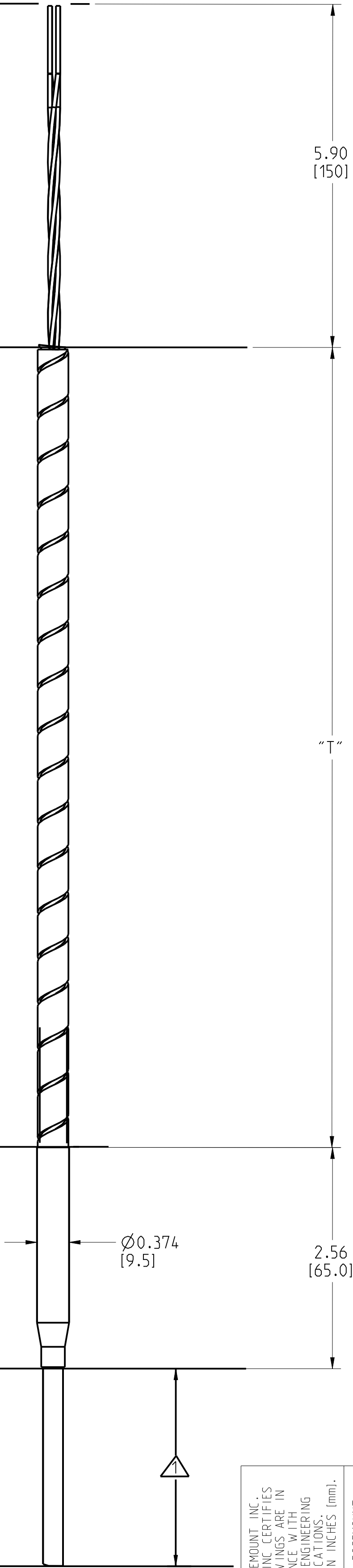
ARMORED CABLE (AN), PVC COATED ARMORED CABLE (AC), PTFE COATED ARMORED CABLE (AP)
