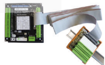
DIN relay card with flat ribbon
