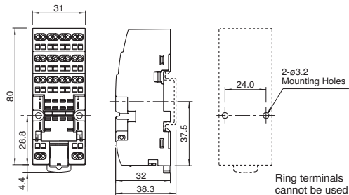
SU4S-11L
