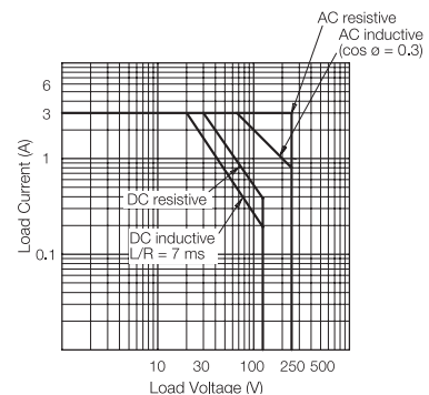
RU42 (Bifurcated)
