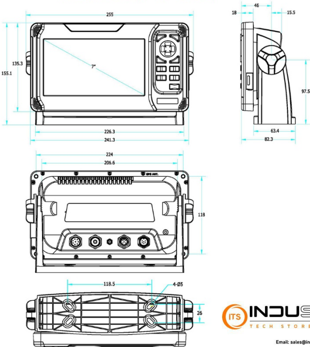
DIMENSIONS (KP-27 SERIES)
