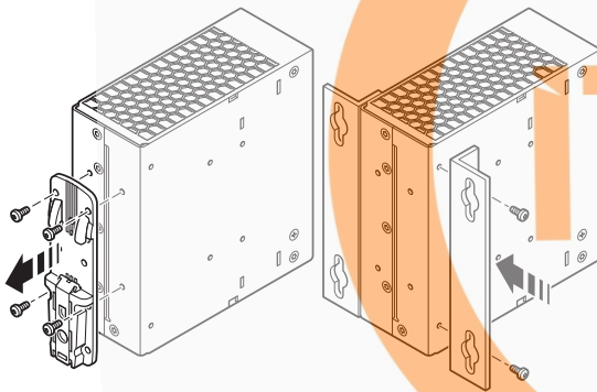
Figure 12 Mounting the UWA 130 universal wall adapter
