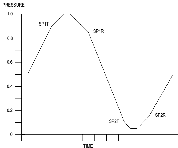
Figure 5: Set points
