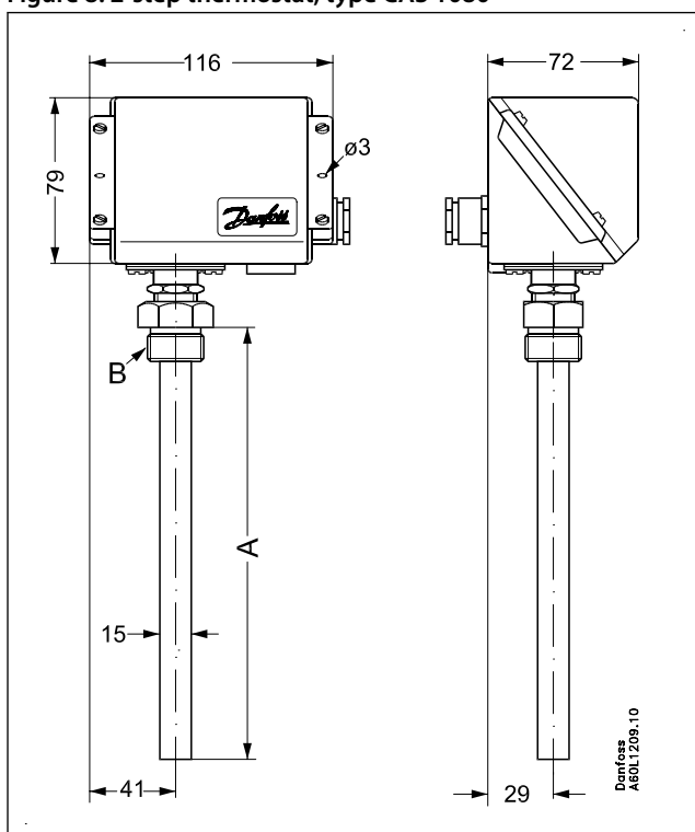
Figure 8: 2-step thermostat, type CAS 1080
