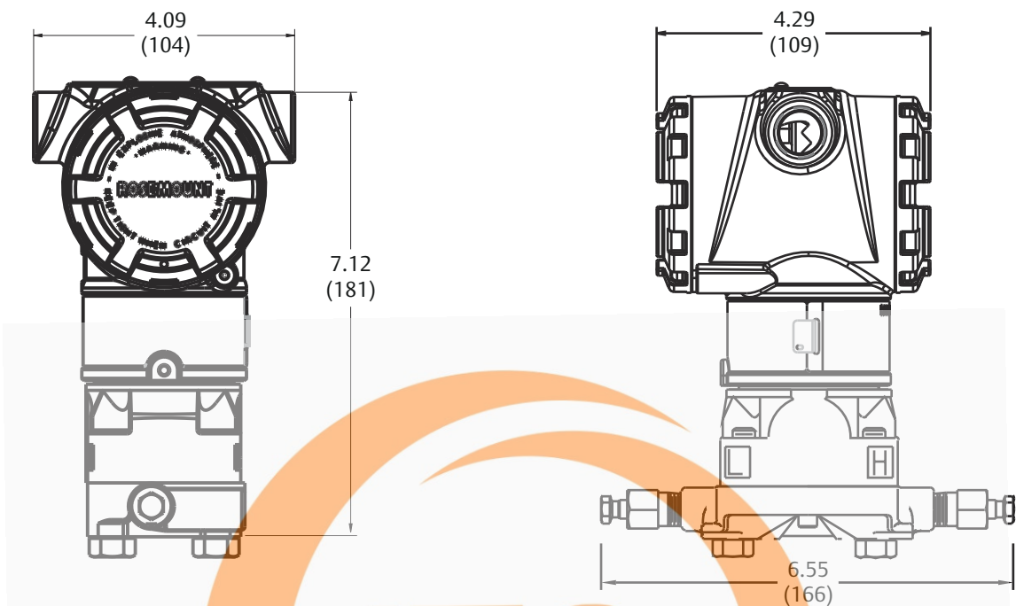
Figure 8: Rosemount 3051C Coplanar Flange
