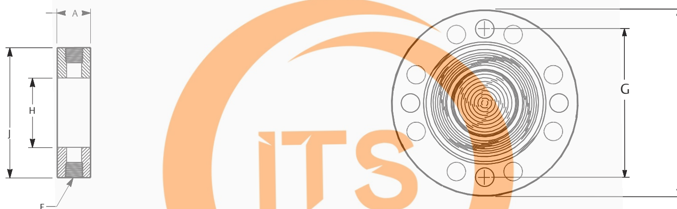
Figure 24: Optional Flushing Connection Ring (Lower Housing) for Rosemount 3051L
