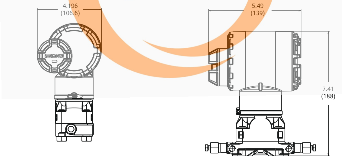
Figure 9: Rosemount 3051 Wireless Housing with Coplanar Flange
