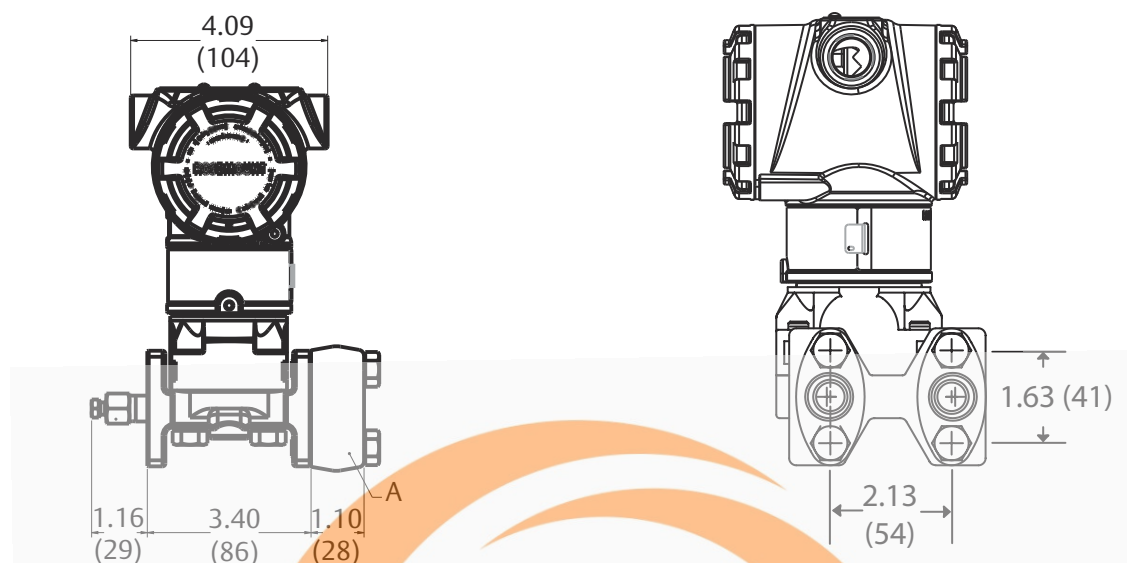
Figure 12: Rosemount 3051C Coplanar with Traditional Flange
