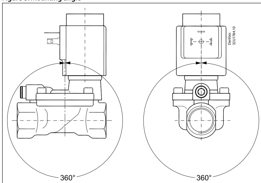
Figure 8: Mounting angle
