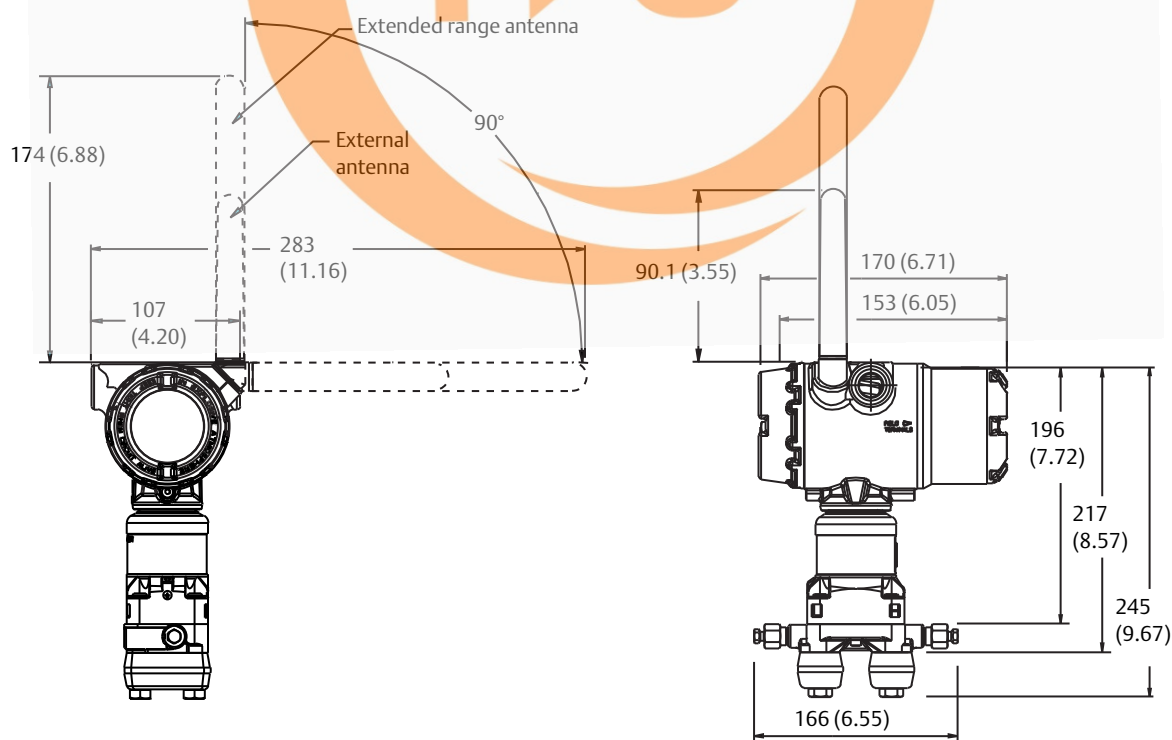
Figure 2. Wireless Version
