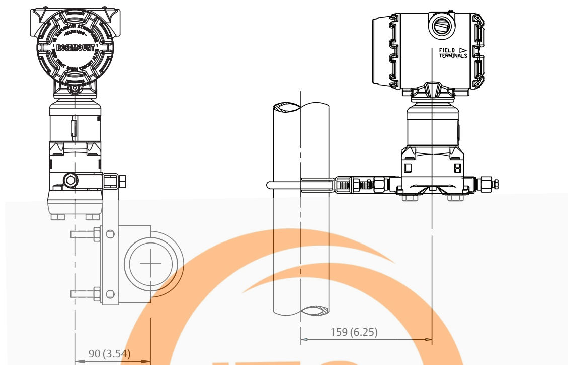
Figure 3. Pipe Installation
