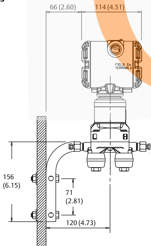
Figure 4. Panel Installation
