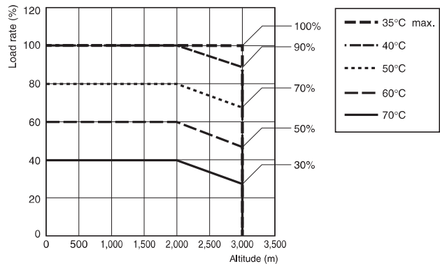
15 W to 150 W (During a DC input)
