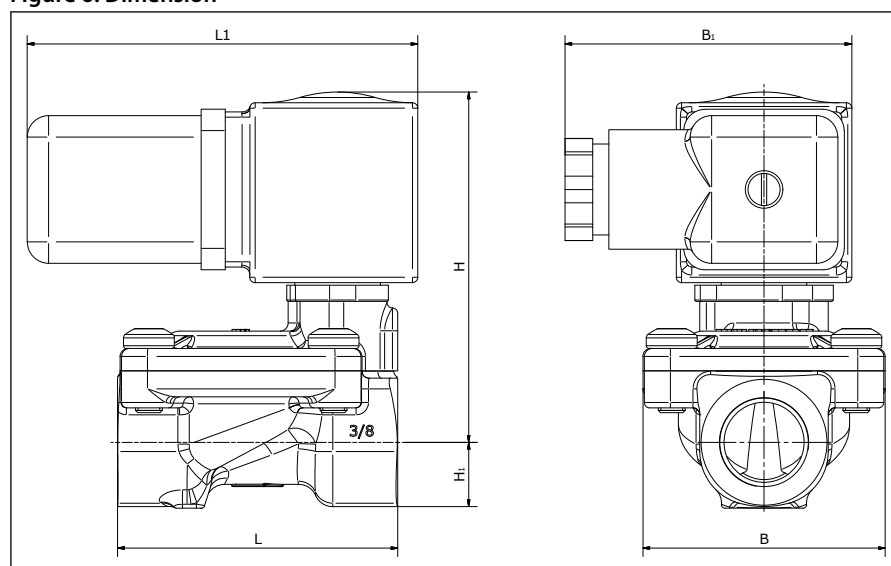
Figure 6: Dimension
