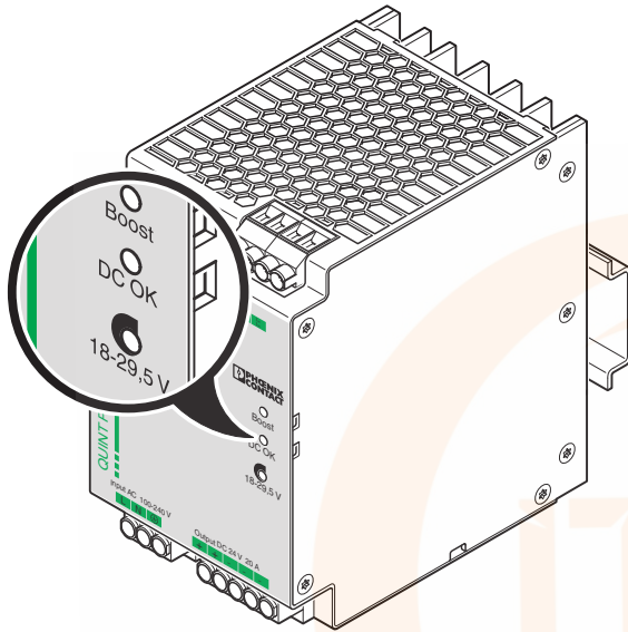
Figure 10 Signal outputs
