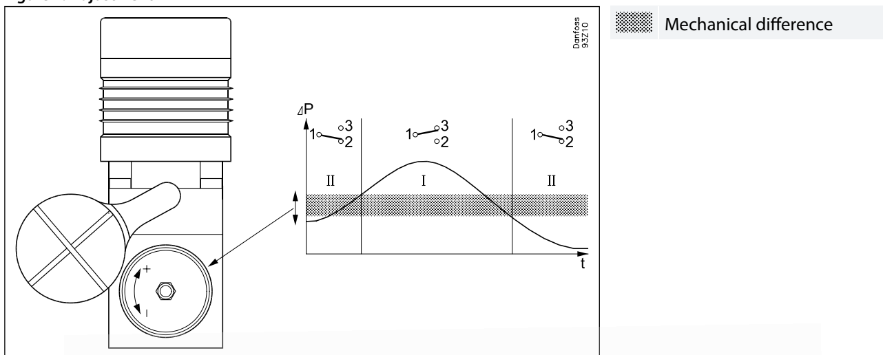
Figure 2: Adjustment
