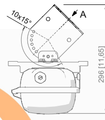
Wall mounting bracket fitted in mounting rail
