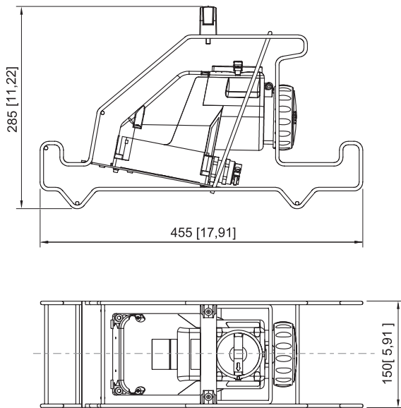
Coupler socket
