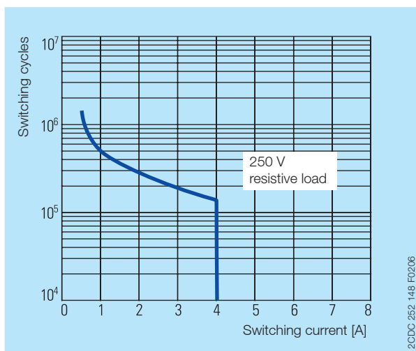
Contact life time / number of operations N 220 V 50 Hz 1 AC, 360 operations/h
