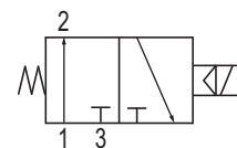
ESV-32 < Normally - open >
