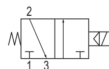
ESV-31 < Normally - closed >
