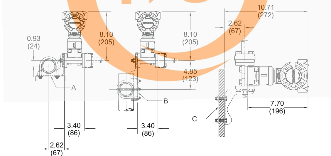
Figure 18: Traditional Mounting Configurations
