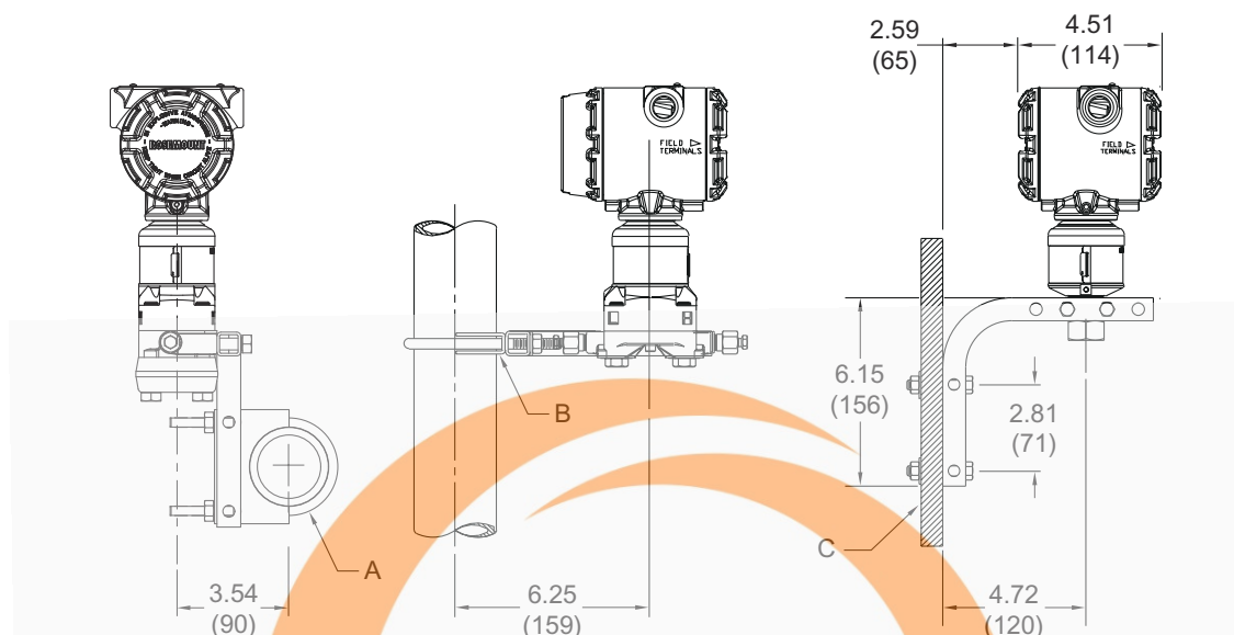
Figure 17: Coplanar Mounting Configurations (B4 Bracket)
