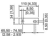
Wall mounting bracket fitted in mounting rail
