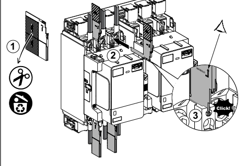
LC1G265-800
