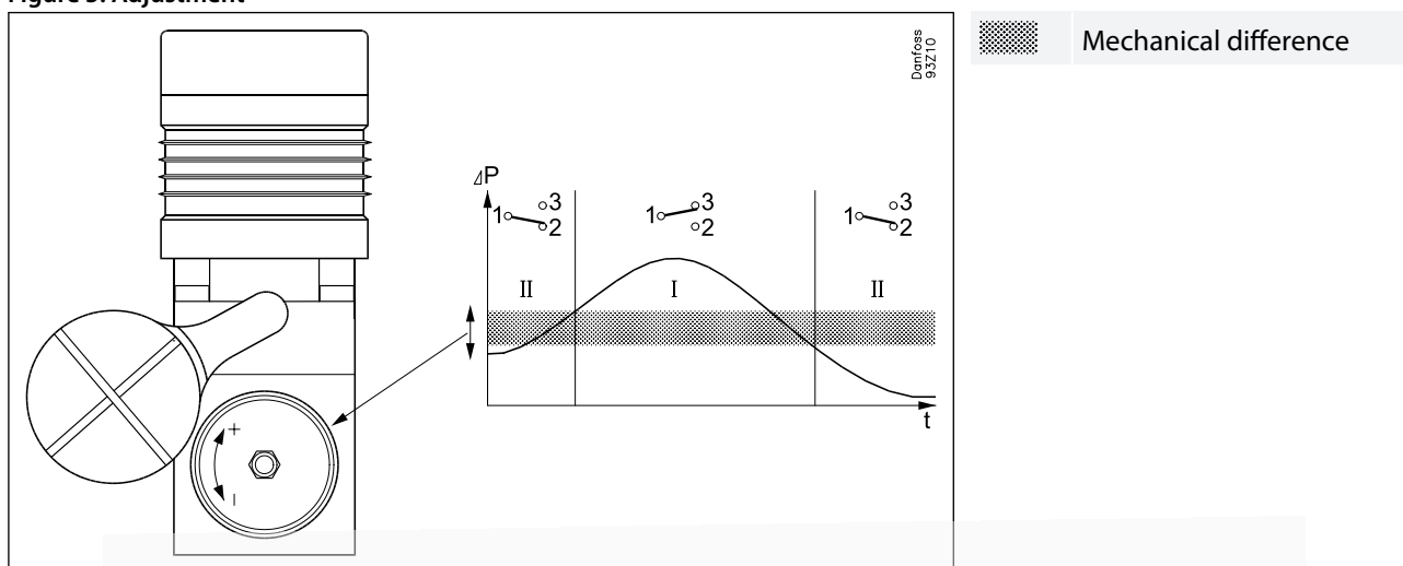
Figure 5: Adjustment
