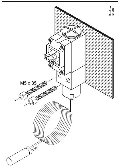
Figure 3: Mounting example
