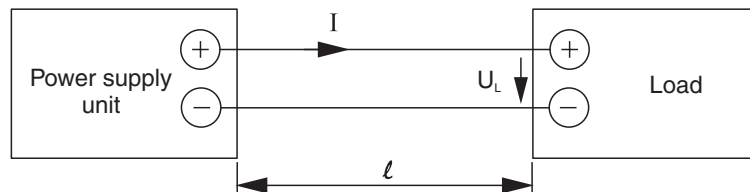
Figure 3-22 Cable length
