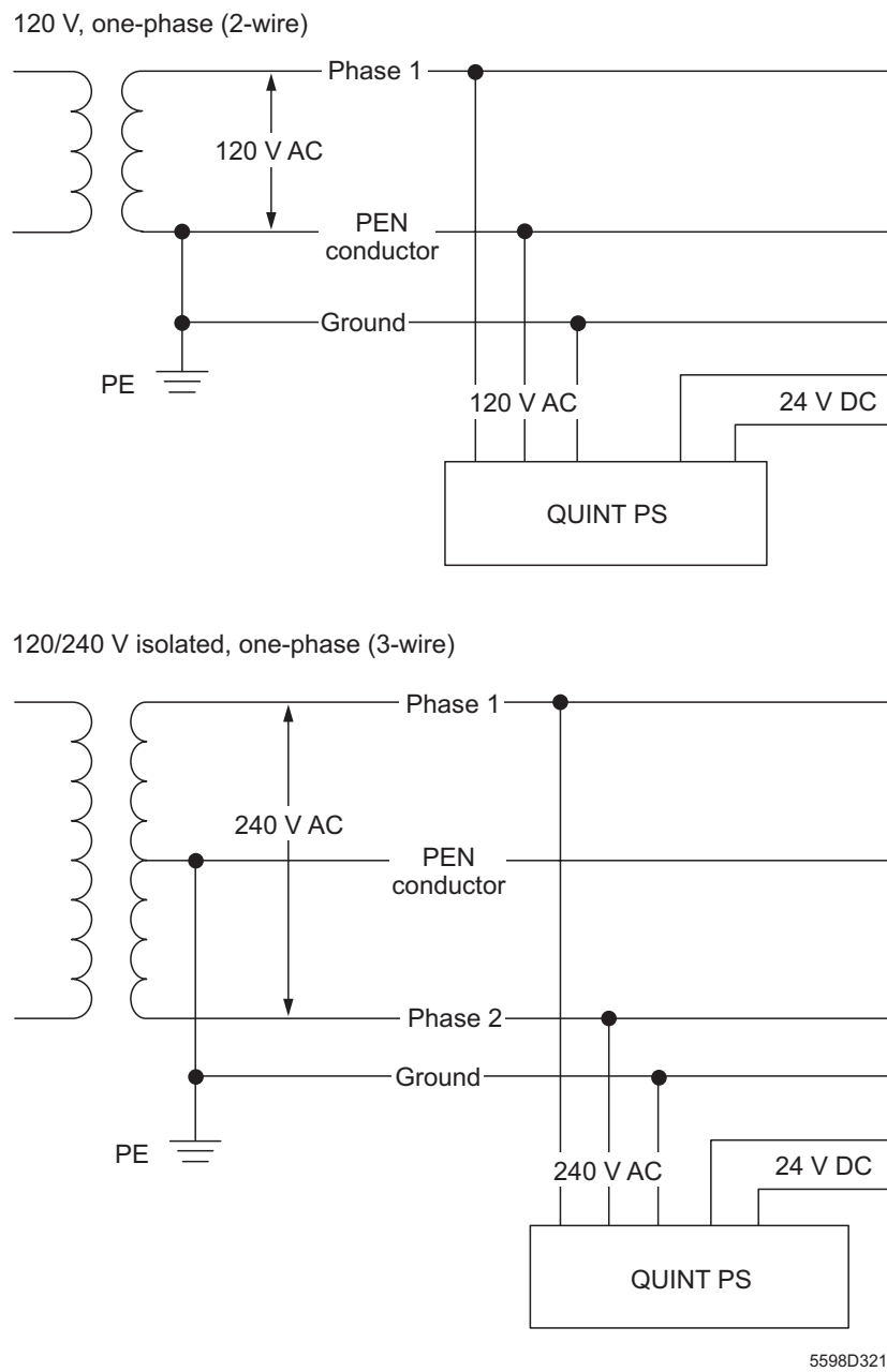
Figure 3-19 US network configurations (one-phase)
