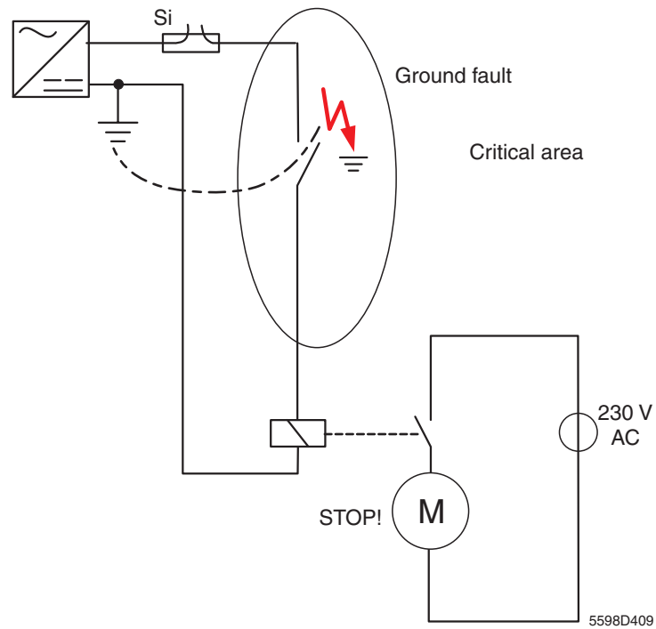
Figure 2-5 With secondary grounding
