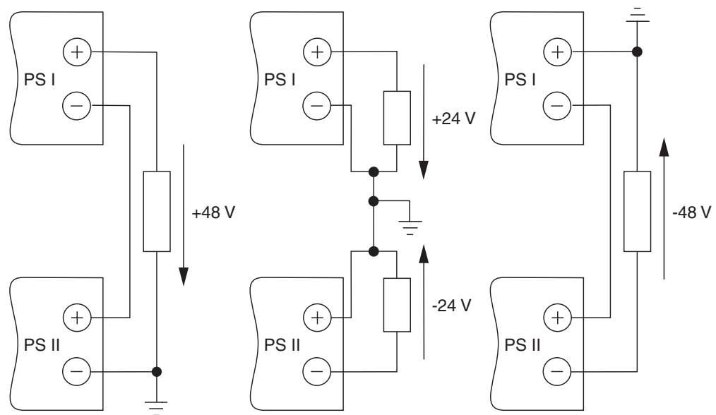
Figure 3-9 Series connection
