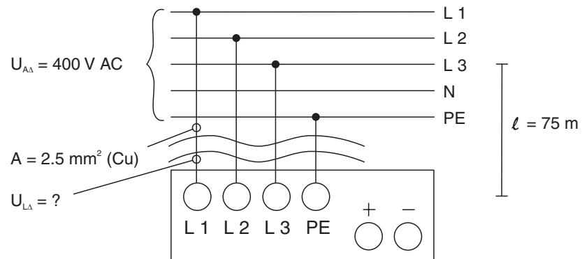
Figure 3-24 TN-S network
