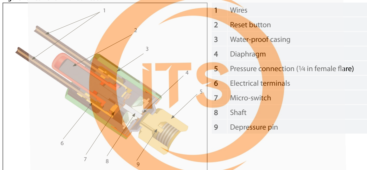
Figure 2: ACB - SPST manual reset
