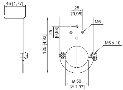
Mounting bracket for surfaces
