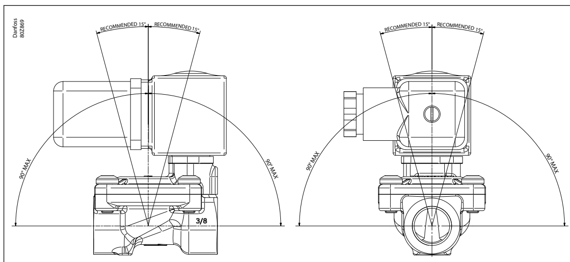
Figure 7: Mounting angle
