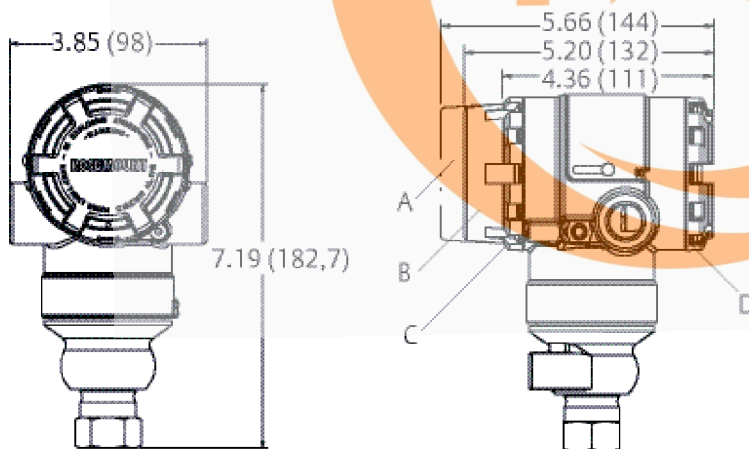
Figure 9: Rosemount 2051T
