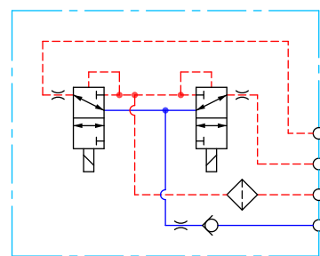
PVEO-R schematic
