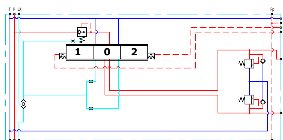
Compensated PVB schematic
