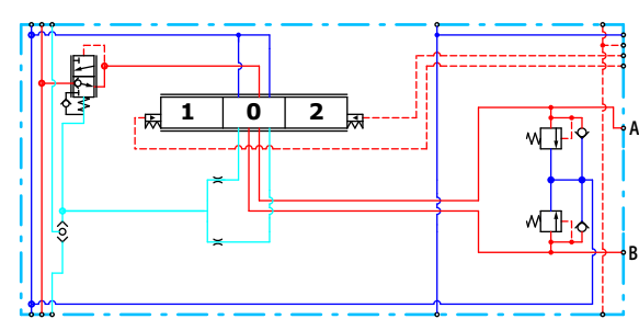
Compensated high flow PVB with T0
