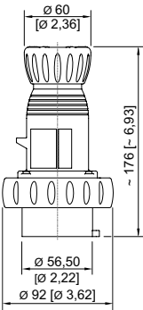
5-pole plug
