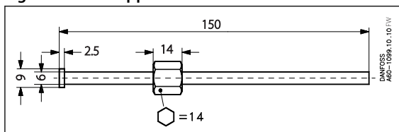
Figure 2: Weld nipple for KP-A
