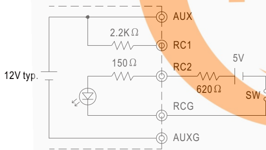
(A)Using external voltage source
