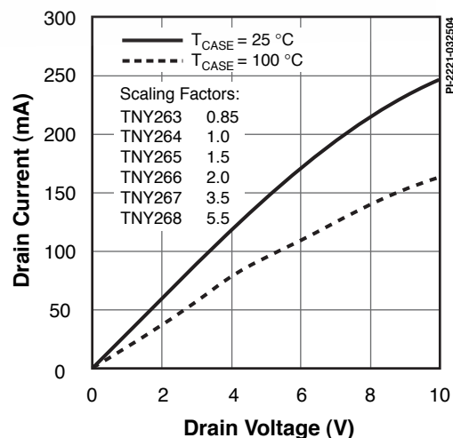
Figure 27. Output Characteristic.
