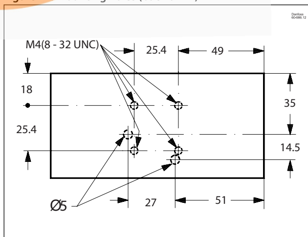
Figure 14: Mounting holes (back of KP)
