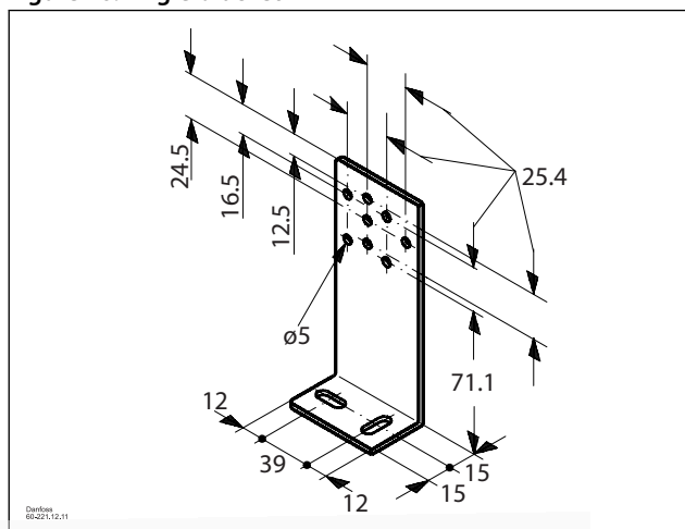
Figure 16: Angle bracket
