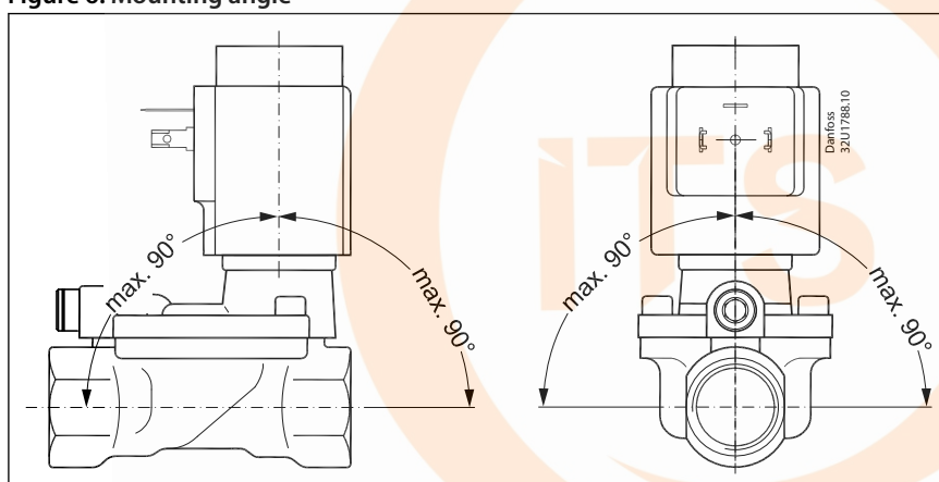
Figure 6: Mounting angle
