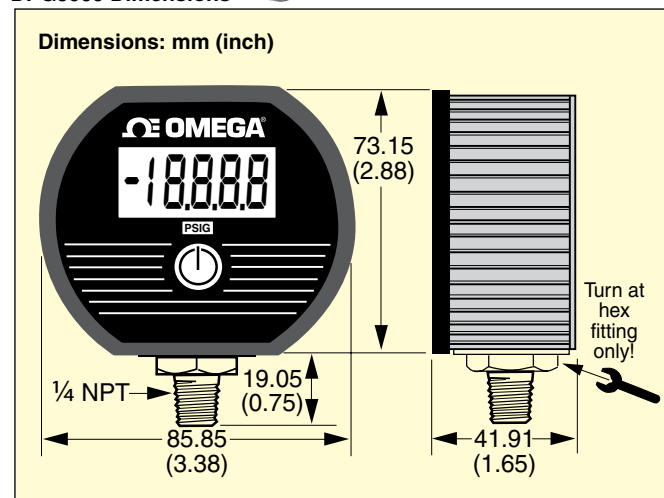
DPG5000 Dimensions
