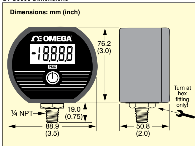
DPG3500 Dimensions
