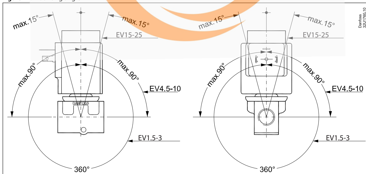
Figure 11: Mounting angle
