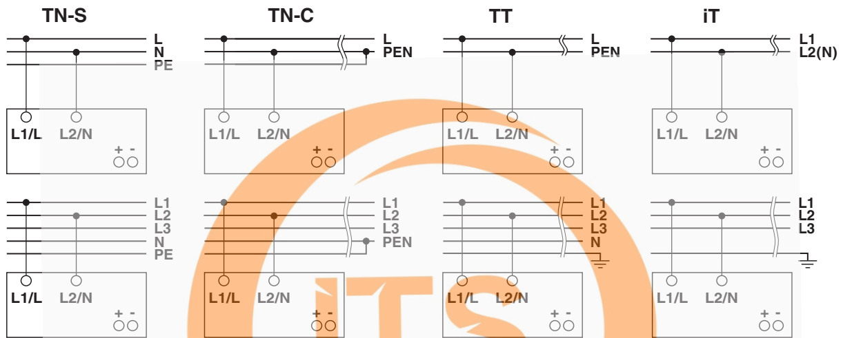
Figure 9 Network types
